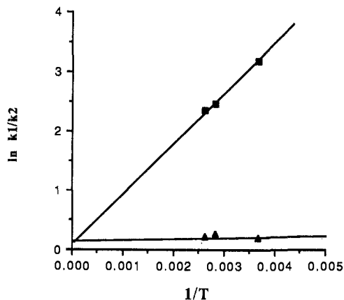
Figure 3. Arrhenius plot of selectivity for addition of cyclohexyl radical to 1 . ■, ln [3b]/[4b]; ▲, ln [5b]/[6b].
