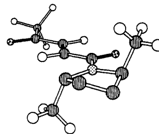
Figure 2. View of low-energy MM2 conformation for alkene 1 . (Pyrrolidine ring hydrogens are omitted for clarity.)
