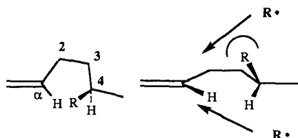
Figure 4. Elements required for \alpha center stereoselection.
